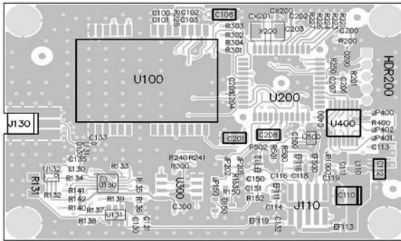
Component Layout
